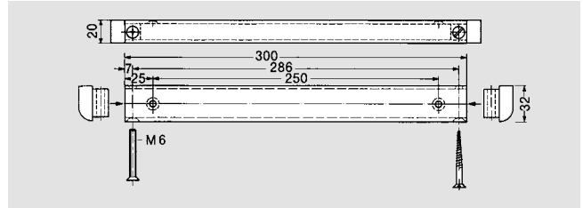
Guide housing Art. No. 7453 N
