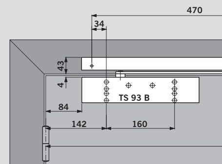
Inactive leaf Minimum width 370 mm in the case of unequal leaves
