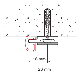
Ceiling mounting with bracket 2150.
