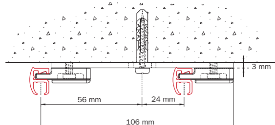
For excellent parallel fitting: mounting with double fixing bracket 2216 and ceiling brackets 2150.
