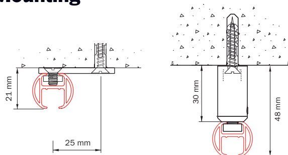
Ceilingmounting 4200 with ceiling bracket 5153
