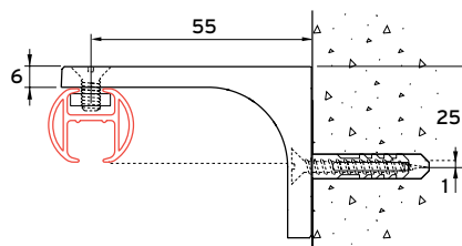
Mounting 4200 with wall bracket 5140
