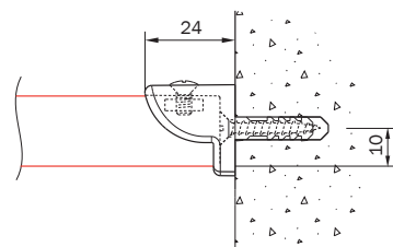
Wall mounting 4200 with wall bracket 4249
