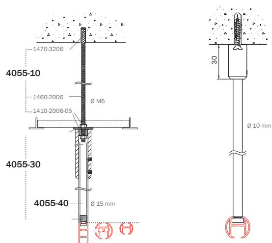
Ceiling mounting 4100, 5100 or 4200: threaded rod set 4055-10, suspension hanger tube 4055-40 and with fixing set 4055-30.
